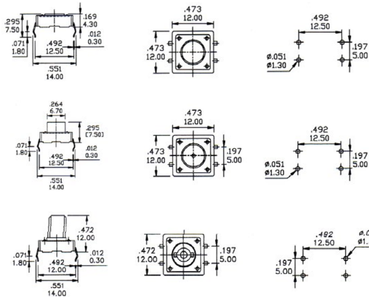
Drilling Patterns
